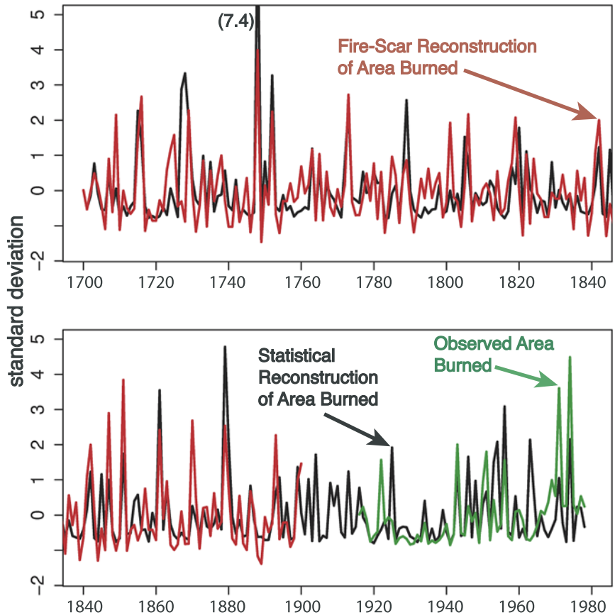
Fig. 1. This comparison shows the statistical reconstruction of the southwestern area burned (1701–1978, black line), the observed area burned for Arizona and New Mexico (1916–1978, green line) used to train the statistical model, and the regional fire-scar index of fire occurrence (1700–1900, red line). Spearman's rank correlation between the observed and statistical reconstruction is 0.49 for the 1916–1978 training period and 0.71 for 1916–1962, prior to the beginning of a four-fold increase in area protected from wildfire. The rank correlation between the statistical reconstruction and the fire-scar reconstruction (1700–1900) is 0.61.
