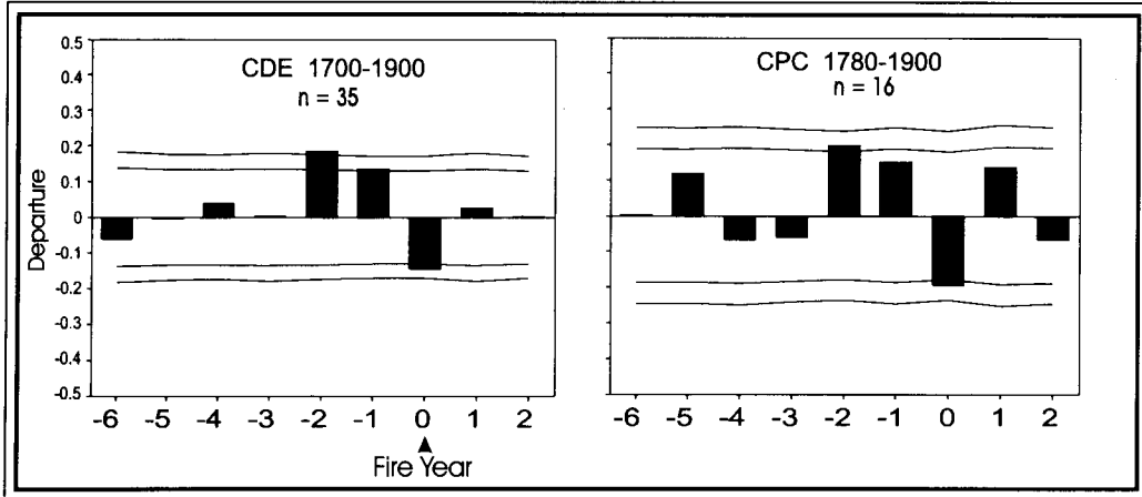
Figure 8 a, b—Plots of superposed epoch analysis comparing estimates of past climate with fire occurrence for periods I and II at the northern fire-history sites (a) and the Manzano Mountain sites (b). The X axis represents a set of nine years, from six years before a fire event to two years following it. Values are averaged at each of these positions for all fire years within the time period analyzed. Confidence intervals are provided by picking a set of dates at random in a thousand simulations. The spread of the confidence bands is greatly affected by the number of events in the simulation (n) that is determined by the actual number which occurred. The data from the Manzanita Mountains show a consistent relationship between drought and fire occurrence, while the La Luz/SNB site shows no relationship between fire and climate during any period. Note the general relationship of fire occurrence on a dry year preceded by one or two wet years at the Manzano sites (CDE and CPC). This pattern is typical of semi-arid forested sites with an open stand structure.
