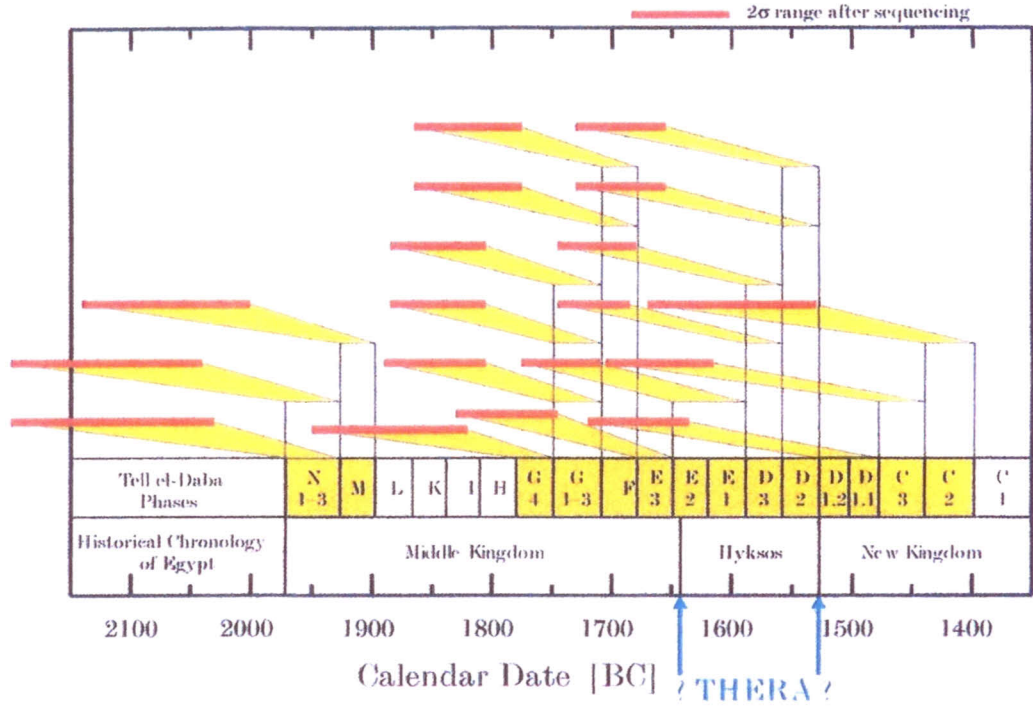
Fig. 2 Comparison of calibrated two sigma ^{14}\text{C} ranges with the historical chronology of Egypt and the corresponding Tell el-Dab'a phases
