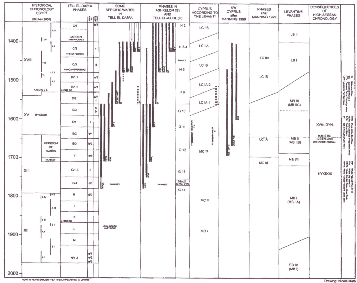
Fig. 1 Comparison of Tell el-Dab'a phases to the chronologies of Ashkelon, Tell el-Ajjul, Cyprus and the Levant, including a reference to the 1645 ±7 Greenland ice-core signal (after BIETAK 2003, fig. 1)
