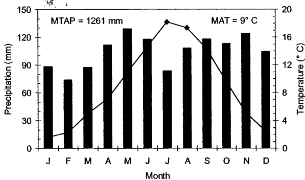
Figure 2. Climograph for Capdella (42°27'55"N, 0°59'28"E, 1270 m elevation, records from 1945 to 1997). Bars indicate mean total monthly precipitation (mm) and solid line indicates mean monthly temperature (°C). MTAP is the mean total annual precipitation and MAT is the mean annual temperature.
