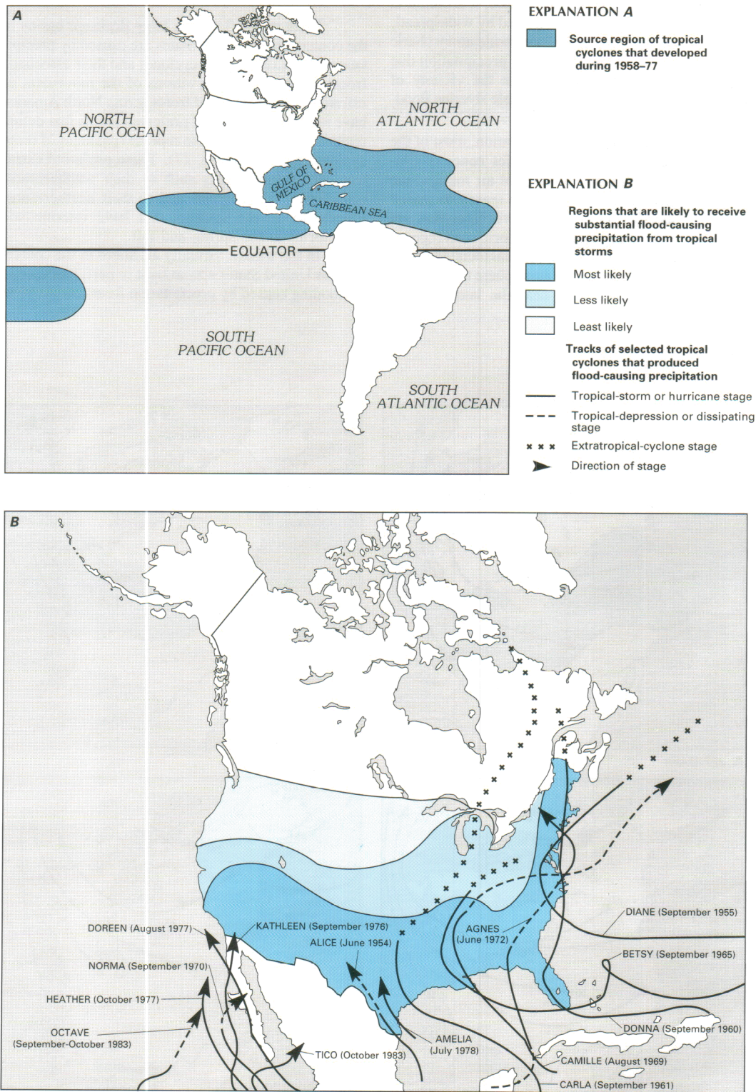
Figure 26. Tropical cyclones and their effect on flooding in the conterminous United States. A , Source regions of tropical cyclones. B , Tracks of selected tropical cyclones that produced flood-causing precipitation or storm surges and regions affected by precipitation from tropical cyclones. (Sources: A , Modified from Gray, 1979; B , Modified from Cry and others, 1981 (tracks in eastern part of map); Smith, 1986 (tracks in western part of map); Cry, 1967 (darker regions in eastern part of map); Smith, 1986 (darker regions in western part of map); Cry and others, 1981 (lighter regions in eastern part of map); Court, 1980 (lighter regions in western part of map).)
