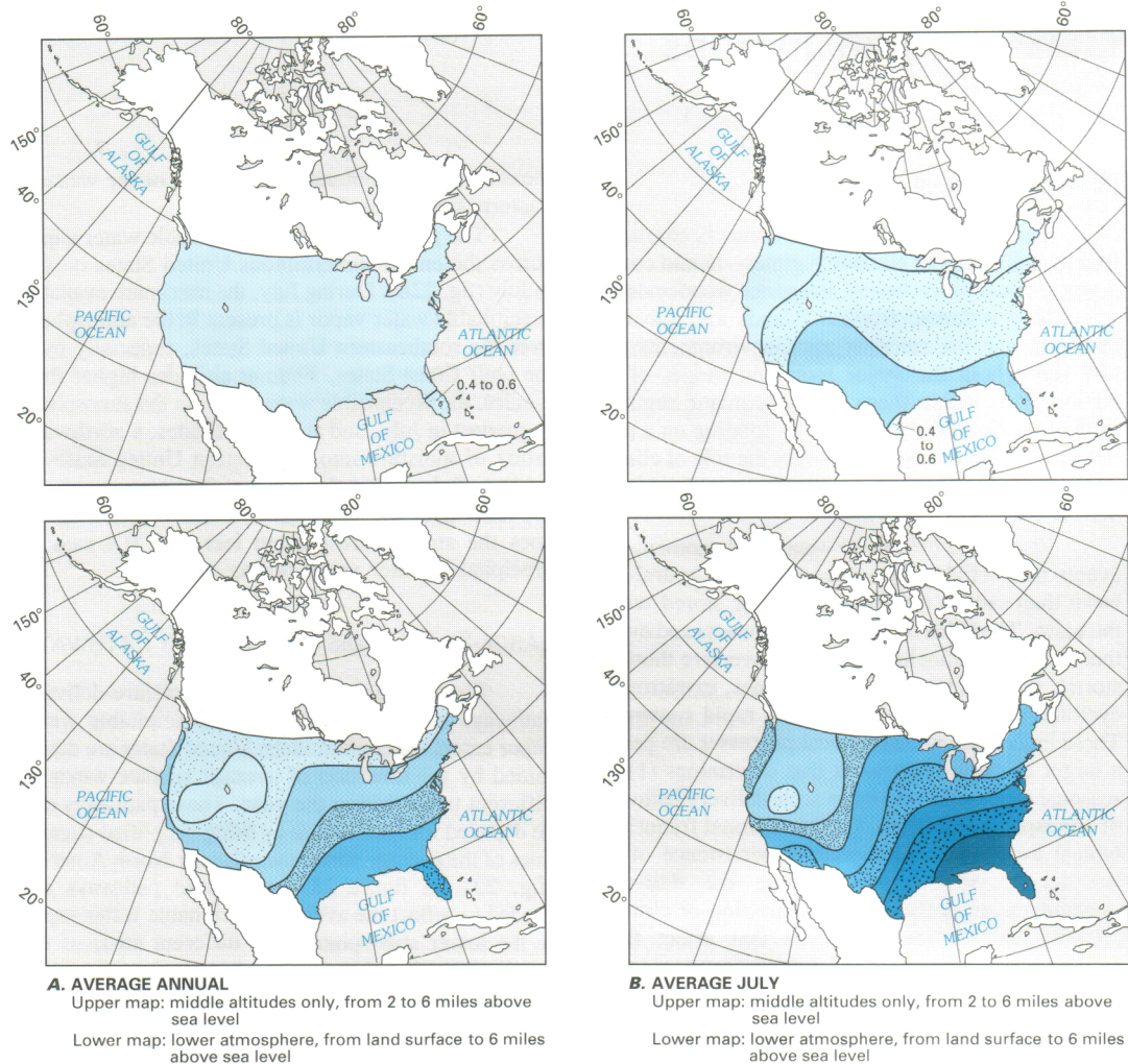
Figure 22. Precipitable water vapor in the atmosphere over the conterminous United States. A , Average annual. B , Average July. (Source: Data from Reitan, 1960.)
