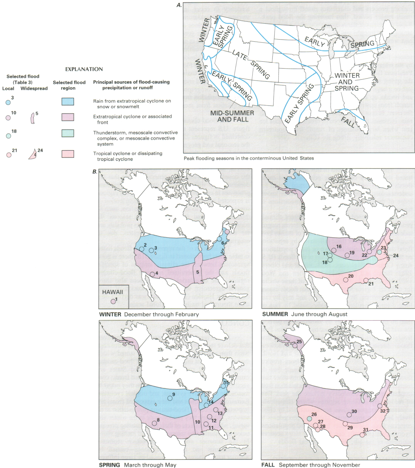
Figure 31. Seasonal summary of flooding and seasonal flood-climate regions in the United States. A. Typical seasons during which the largest flood peak of the year occurs in different parts of the conterminous United States. B. Seasonal flood-climate regions in the United States and selected examples of floods caused by different sources of precipitation or runoff. (Sources: A. Modified from Baldwin and McGuinness, 1963. B. Information presented in this article.)
