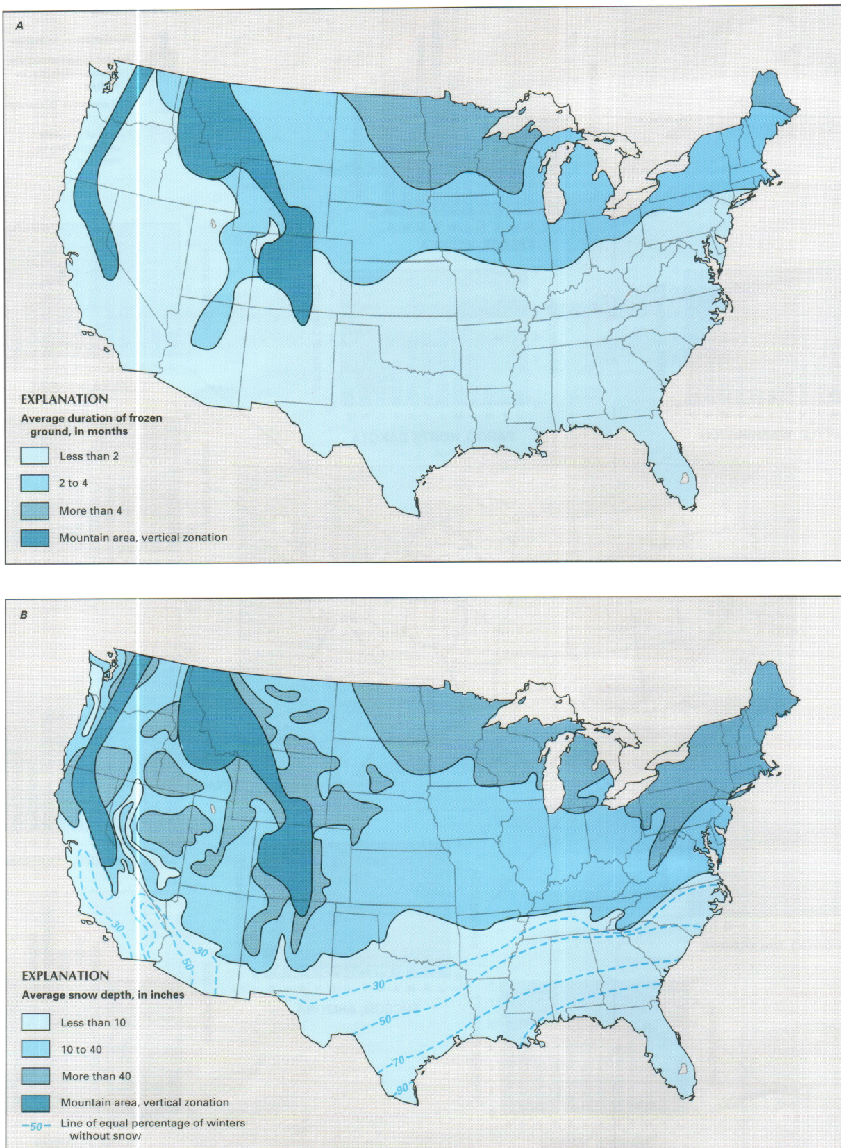
Figure 30. Average duration of frozen ground (A) and average snow depth (B) in the conterminous United States. (Source: Data from Rabenhorst, 1981.)
