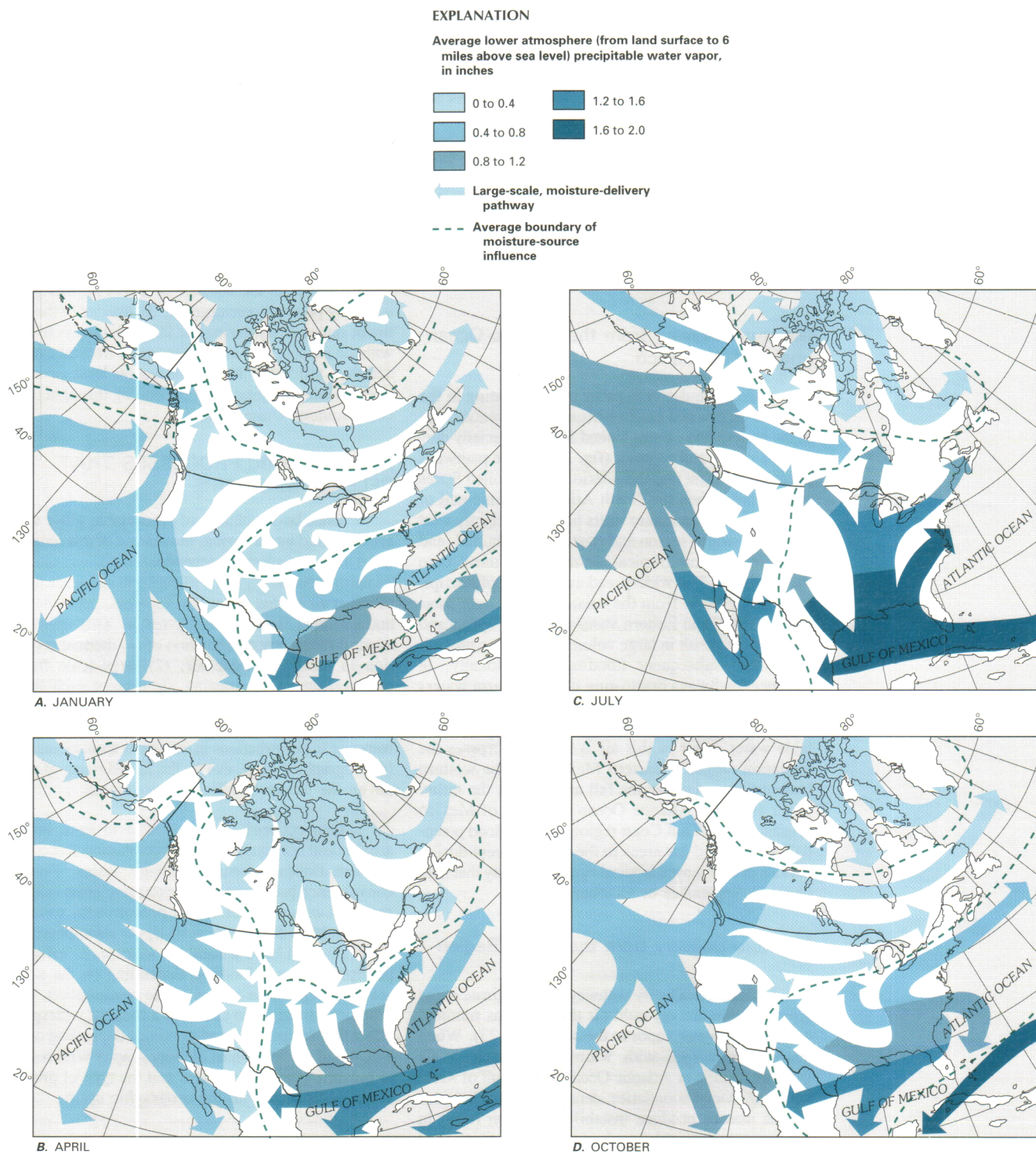
Figure 23. Large-scale, moisture-delivery pathways over North America in four midseason months. (Sources: Pathways data from Bryson and Hare, 1974; precipitable water vapor data from Reitan, 1960.)
