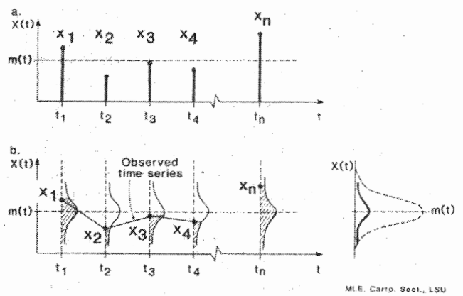
FIGURE 13. The standard stationary stochastic process model for a flood series. (a) Generalized version of an observed flood series. (b) Conceptual representation of the stationary stochastic process with time invariant mean and variance (modified from Kisiel, 1969a).
