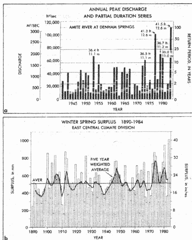
FIGURE 11. Use of the water budget for interpreting streamflow variability. (a) Annual and partial flood series for the Amite River in eastern Louisiana. Partial series peaks are shown with white horizontal bars. Most of the annual floods occur in spring. A trend toward larger floods is evident in recent years. Nonclimatic factors, such as land-use changes or measurement error, are often proposed as explanations for trends like this one in a flood series. (b) Time series of the winter–spring surplus available for runoff in east-central Louisiana, computed from climatic data. The plot shows that the 11-yr period between 1973 and 1983 was extremely wet in winter and spring and generated some of the largest seasonal moisture surpluses in the entire 96-yr record. This additional hydroclimatic information lends support to a climatic explanation for the recent trend toward increasing flood peaks (Source: Muller and McLaughlin, 1987).
