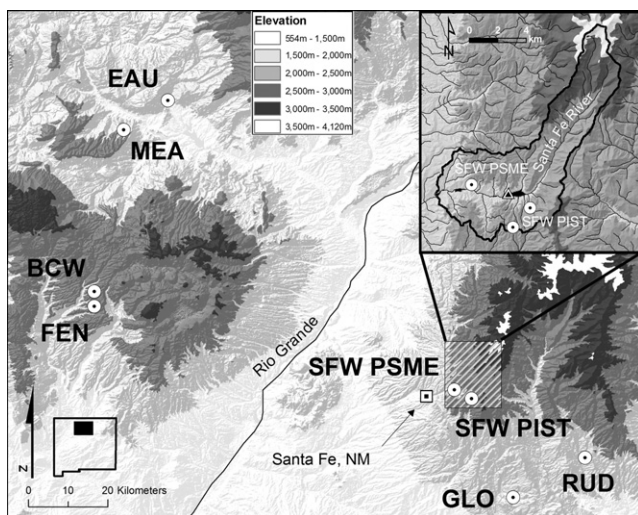
Fig. 1. Location of tree-ring sites (circles) and upper Santa Fe River watershed (hatched box) in northern New Mexico. (Inset) Tree-ring sites and Santa Fe River near Santa Fe gage location (triangle) within the watershed.
