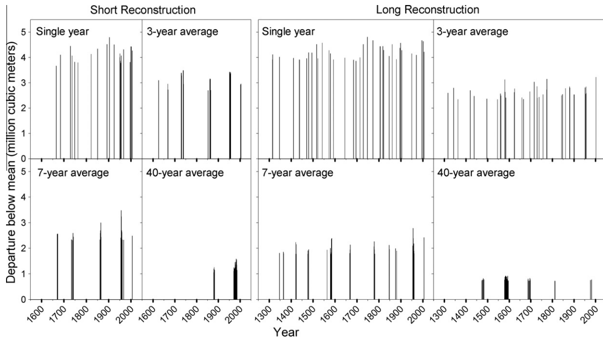
Fig. 5. Time plots of reconstructed extreme (5th percentile) dry events: lowest single-year flows and running means of indicated length. (Left) Short reconstruction, 1592–2007. (Right) Long reconstruction, 1305–2007. Flows plotted as departure below respective reconstructed instrumental-period (1914–2007) mean annual discharge (short reconstruction, 6.91 MCM; long reconstruction, 6.54 MCM). Running averages plotted on last year.
