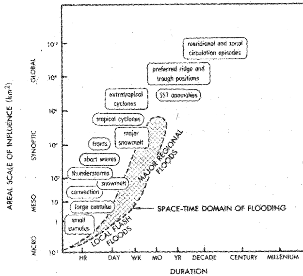
FIGURE 1. Space-time domain for selected meteorologic, climatic, and hydrologic phenomena. The spatial domain is represented by the typical areal scale of influence of each phenomenon, in kilometers squared. The temporal domain is represented by the typical duration of each phenomenon.
