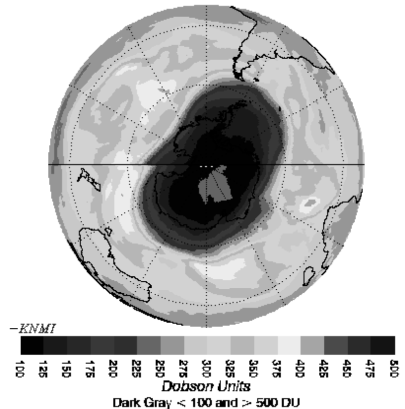
OMI Total Ozone for Oct 8, 2006
