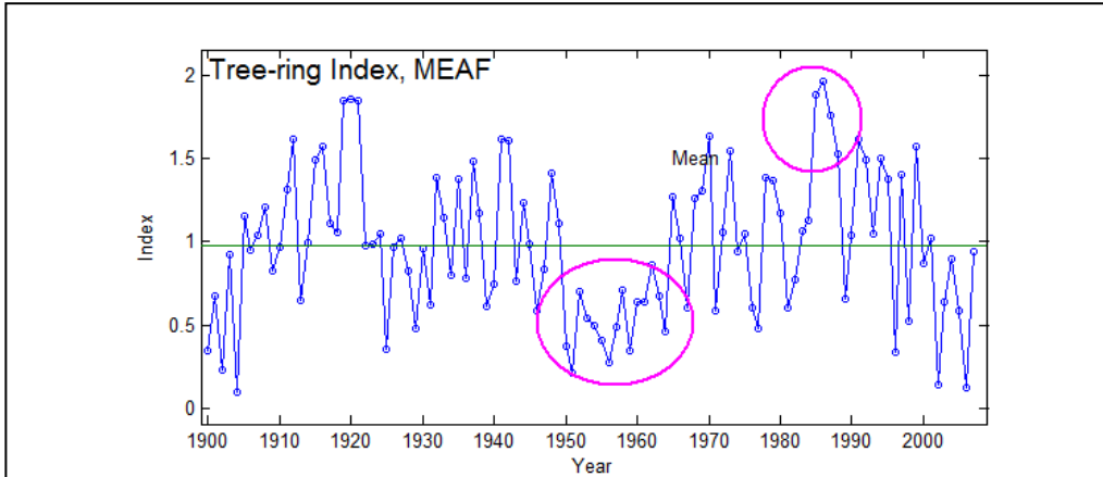
Figure 3.1. Time series plot illustrating signatures of persistence. Tendency for highs to follow highs or lows to follow lows (circled segments) characterize series with persistence, or positive autocorrelation.
